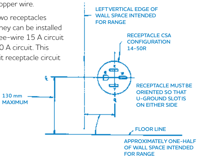
Range receptacle installation - Figure 2
